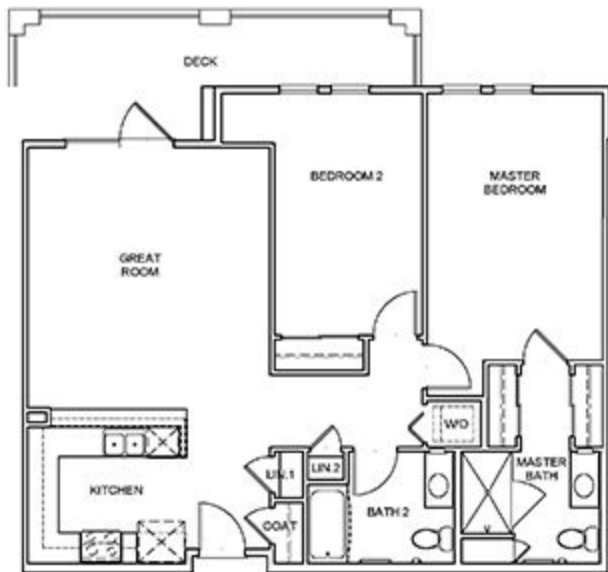
PLAN 2d UNIT #18 2-BEDROOM
