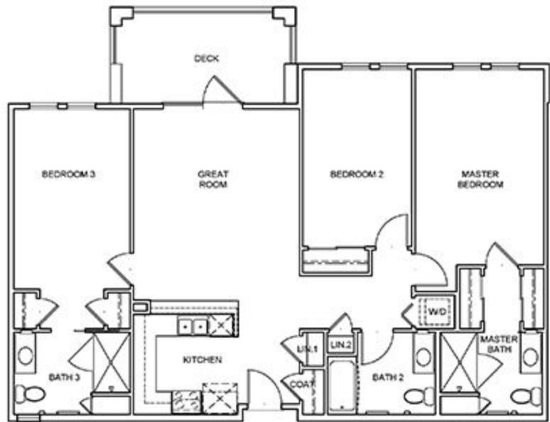
PLAN 6A UNIT #11 3-BEDROOM
